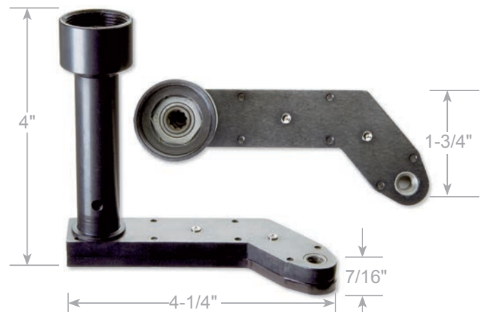
Weight .9 Lbs. Flat Offset 4" Dogleg Right PART #90-041
